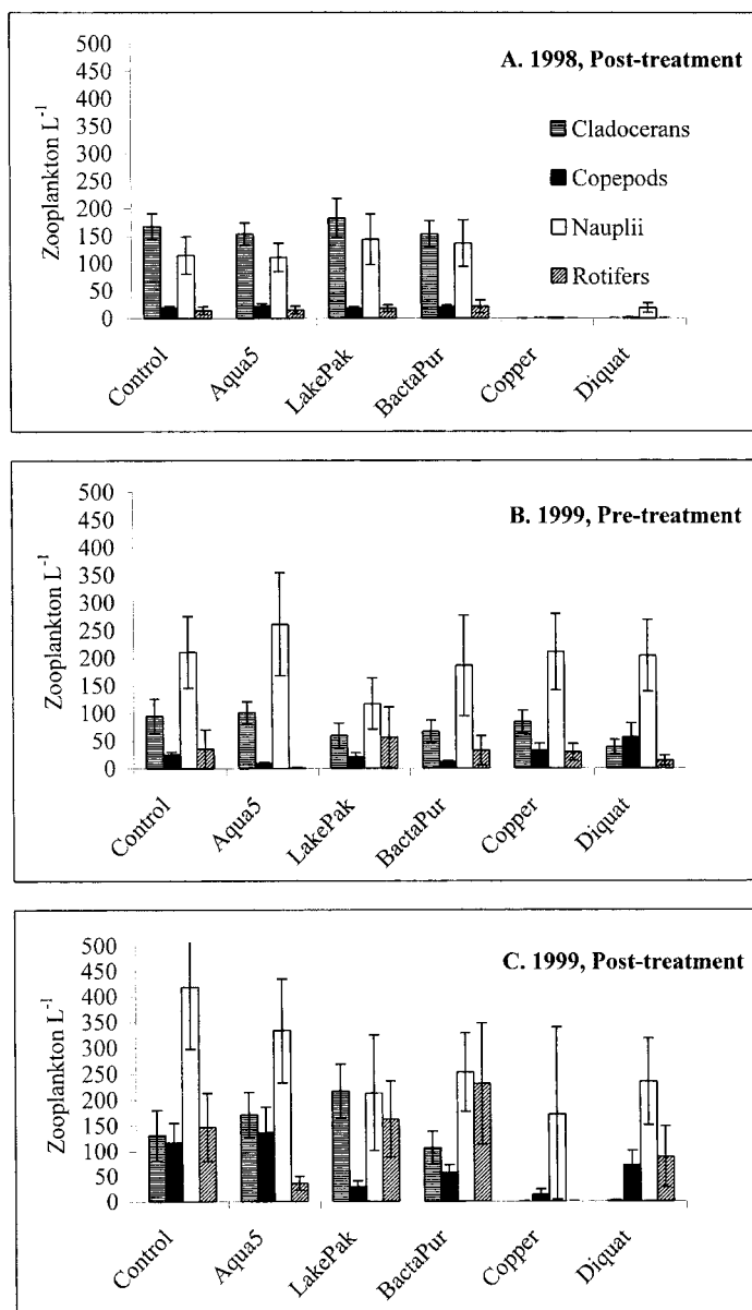
Figure 3. Mean zooplankton abundance in 100-L enclosures (A) one month post-treatment fall 1998, (B) pre-treatment spring 1999 and (C) one month post-treatment spring 1999. Bars indicate standard errors of the mean, N = 16 .
